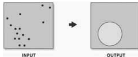
Figure 4: The standard distance is represented as a circle centered on the mean center, with a radius equal to the standard distance (ESRI ArcGIS Resource center 14 ).
