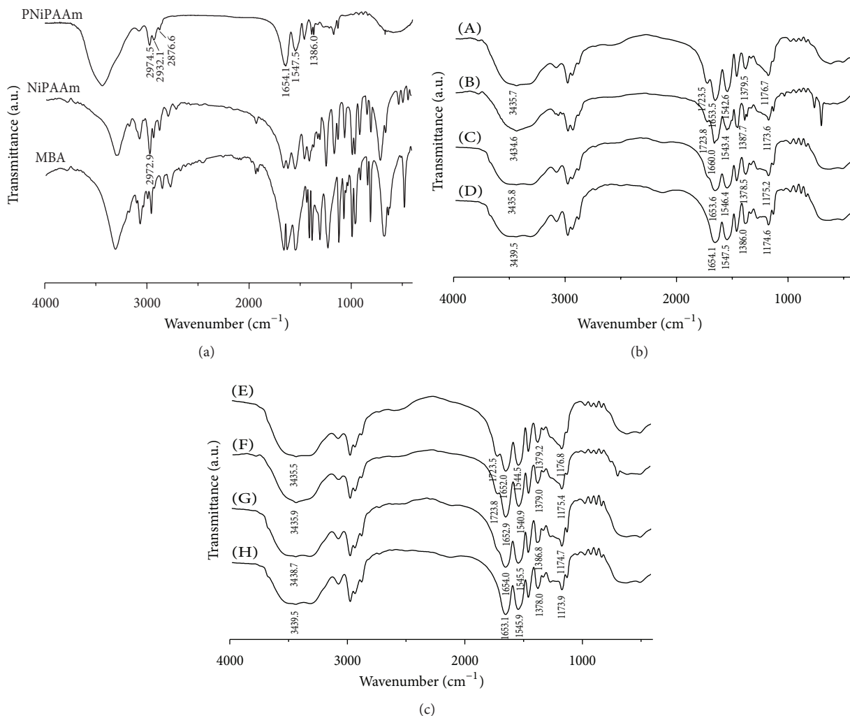
FIGURE 1: FT-IR spectra of hydrogels: (a) spectra of PNiPAAm, NiPAAm, and MBA; (b) spectra of hydrogels with 2.0 wt.% of MBA ((A) 85/15/2; (B) 90/10/2; (C) 95/5/2; (D) 100/0/2); and (c) spectra of hydrogels with 4.0 wt.% of MBA ((E) 85/15/4; (F) 90/10/4; (G) 95/5/4; (H) 100/0/4). The first two numbers in the sample labels correspond to the comonomer NiPAAm/IA weight ratio, and the third one corresponds to the concentration of the crosslinking agent, MBA.
