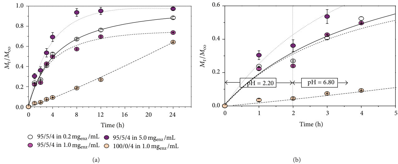
FIGURE 6: Mean normalized cumulative values of released lipase ( M_t/M_{\infty} ) as a function of time at 37°C for hydrogels P(NiPAAm/IA) with 4.0 wt.% of the crosslinking agent. Each data point is calculated based on at least three measurements.
